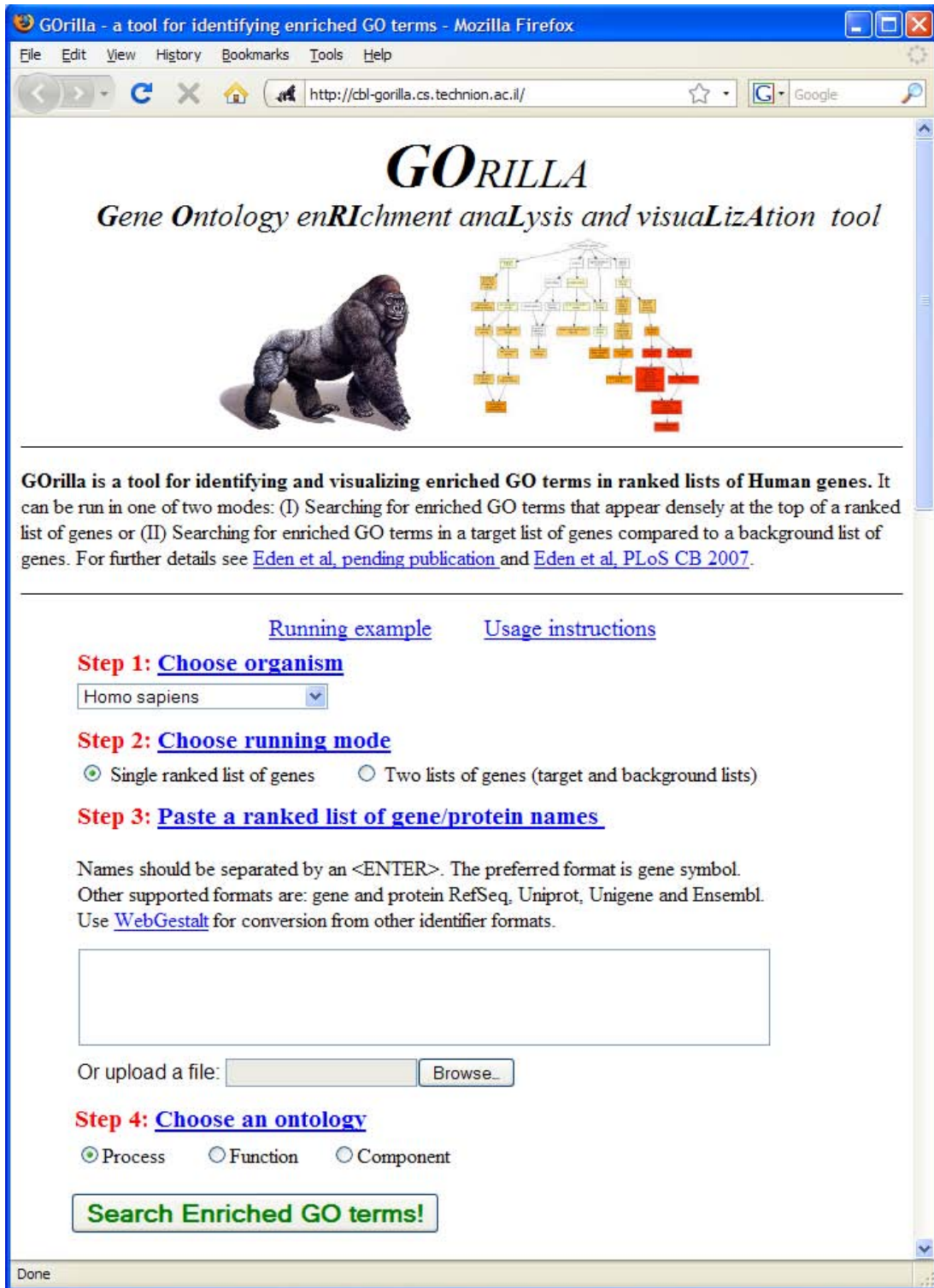
Figure 1 How to use the GORilla web user interface. To use the GORilla web interface, the user is required to perform the following four simple steps: (i) choose an organism; (ii) choose a running mode (either flexible threshold or fixed threshold mode) (iii) copy and paste a list (or upload a file) of genes in the case of a flexible threshold or two lists of genes – a target and a background – in the case of a fixed cutoff; (iv) choose an ontology.
